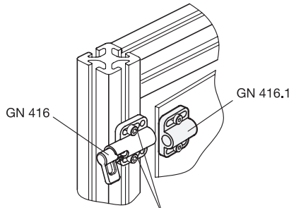
Assembly set GN 965 / GN 968
