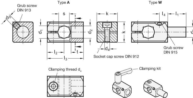
3 Type A with bore W with bolt
