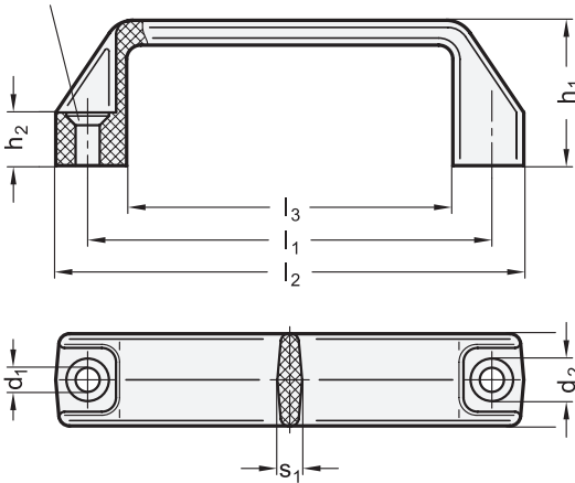
GN 528.2 Bore for countersunk screw DIN 7991
