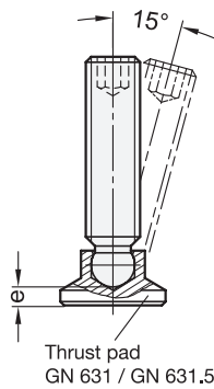
Mounting example
