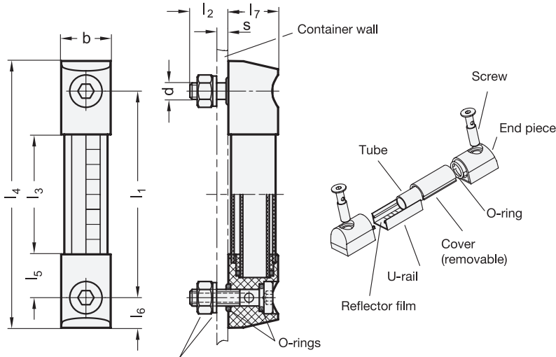
ELESA original design HCK./HCK-GL
