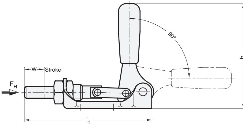
2 Type AS Sheet metal body
