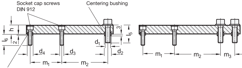
2 Centering guide bushings GN 870
