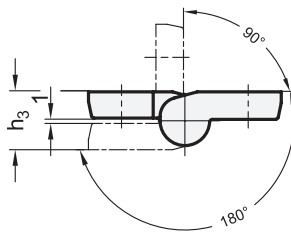
Swivelling range
