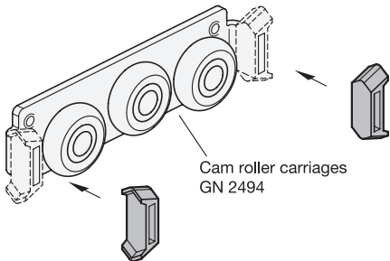
Mounting example
