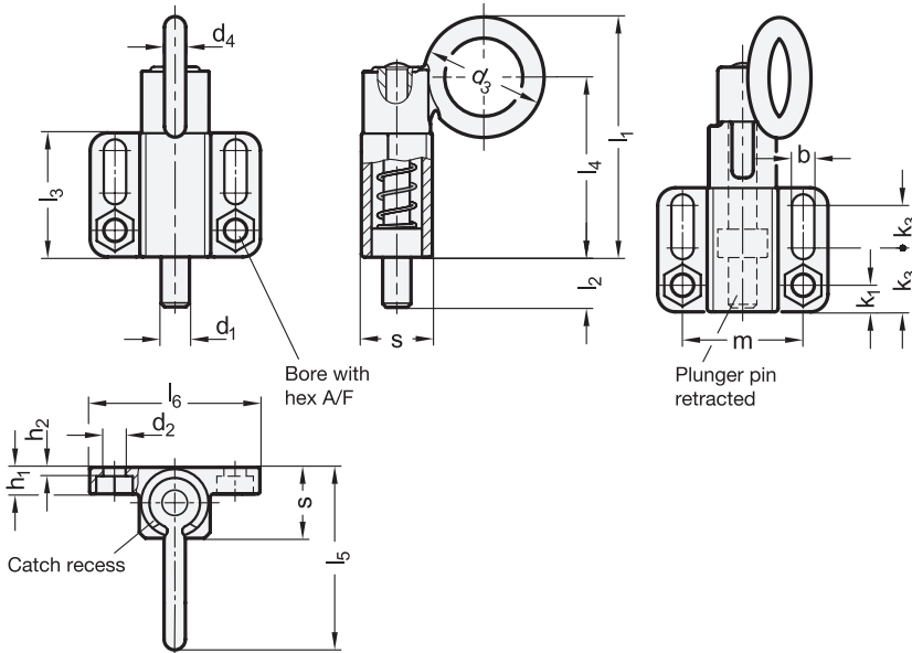
3 Type C With pull ring, with rest position
