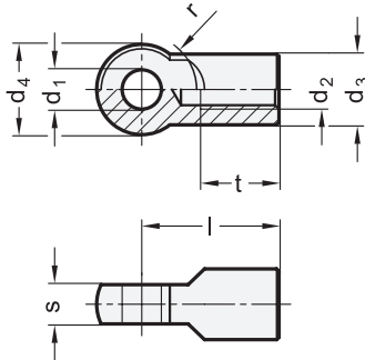
Fork joint GN 751
